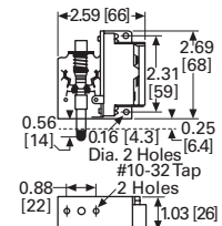
Cabinet Door Type One Contact Block
