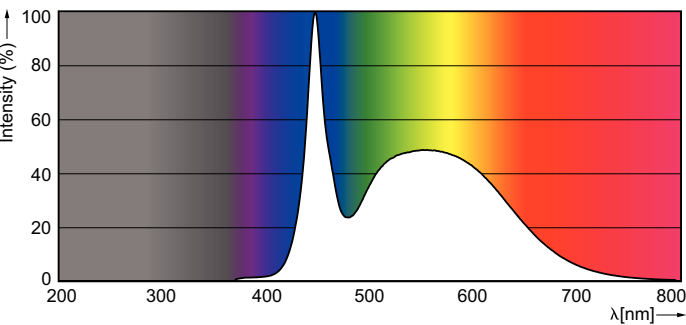
LEDtube 1200 mm 21 W, 865, G13, T8, UO
