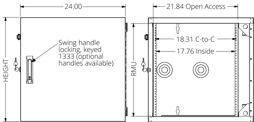
FRONT VIEW WITH DOOR
